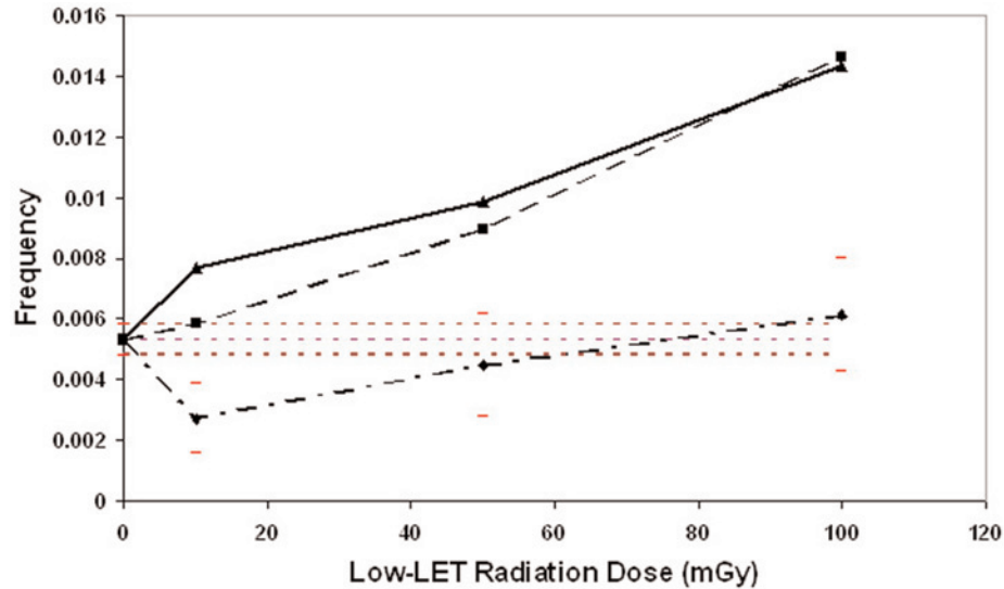
FIGURE 1. Dose-response curves for the frequency of micronucleated cells after exposure of human lymphocytes to photon radiations with different energy characteristics: Gamma rays (diamonds); 70-kVp X rays (squares); 250-kVp X rays (triangles). Horizontal dashed lines indicated the 95% confidence region for the pooled control data. Error bars for data points are 95% confidence intervals.
