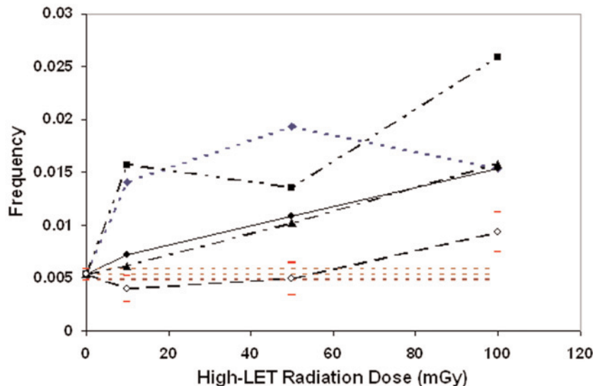
FIGURE 2. Dose-response curves for the frequency of micronucleated cells after exposure of human lymphocytes to monoenergetic neutrons: 13.7-MeV (open circles); 1.5-MeV (triangles); 5.9-MeV (closed circles); 0.44-MeV (squares); 0.22-MeV (diamonds). Horizontal dashed lines indicated the 95% confidence region for the pooled control data. Error bars for data points are 95% confidence intervals.
